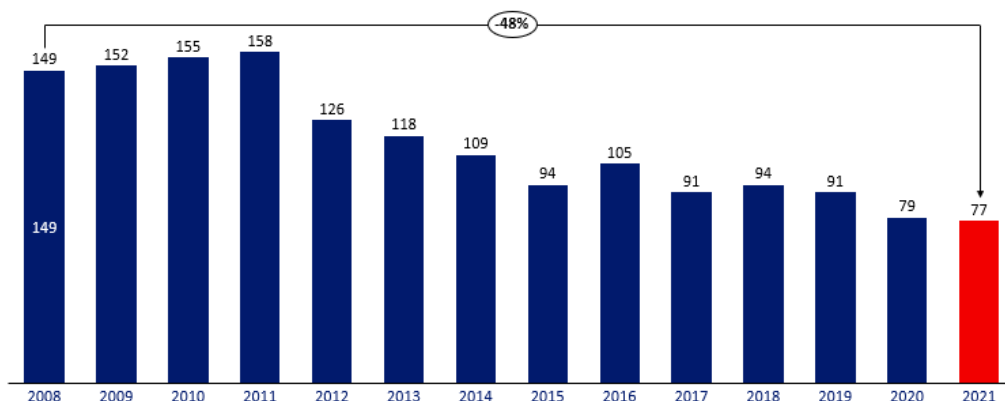
Fuel burn per seat 2008-2021 Scheduled service (Kilo/seat)
